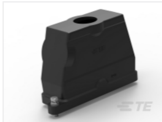
TE Part # T1926240142-001 H24BPR-TGH-4S-PG42
