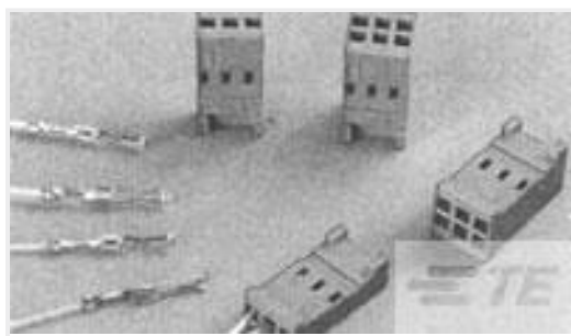
TE Part #1-281838-0 HOUSING HE13 HE14 COSI 10 P
