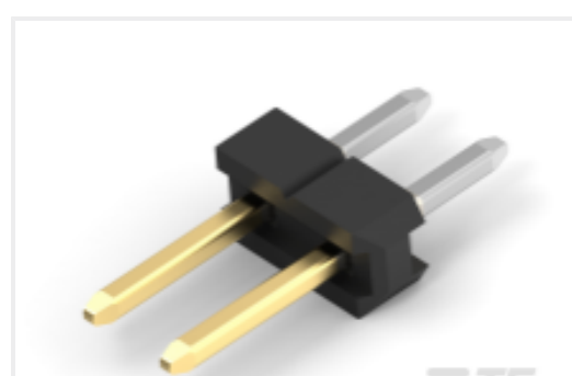
TE Part #2823088-2 2P,2MM,BRK HDR,SRVT,2.8,0.76AU,TB
