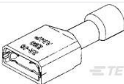
TE Part #2-520103-2 ULTRAFAST 250 ASSEMBLY TAB 22- 18 AWG BR
