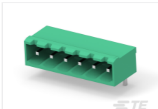
TE Part #2350513-6 6POS TB HDR 90 DEG, PITCH 5.0 & TL 4.5mm
