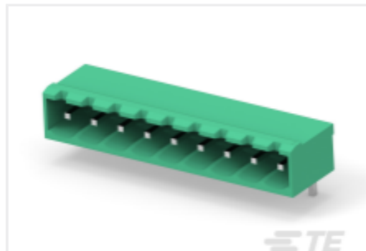
TE Part #2350513-9 9POS TB HDR 90 DEG, PITCH 5.0 & TL 4.5mm
