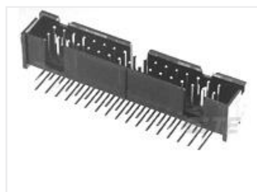
TE Part #5103311-8 A/L LOW PRO HDR 40P RA BLACK
