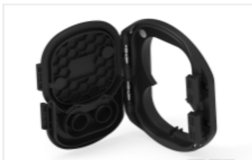
TE Part #2358664-6 FLAP, ASSY, INLET COMBO 2, LEFT, LED
