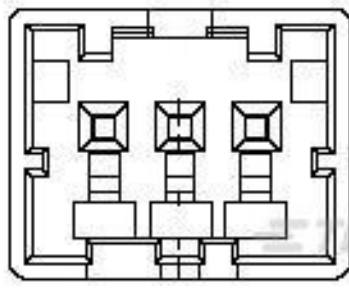
TE Part #1903392-1 GIC 2.5 W CAP HSG 3P NATURAL
