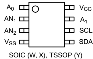
SOIC 8 CASE 751BD
