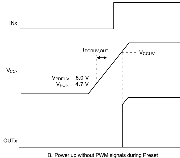
Figure 55. V CCX Power-up
