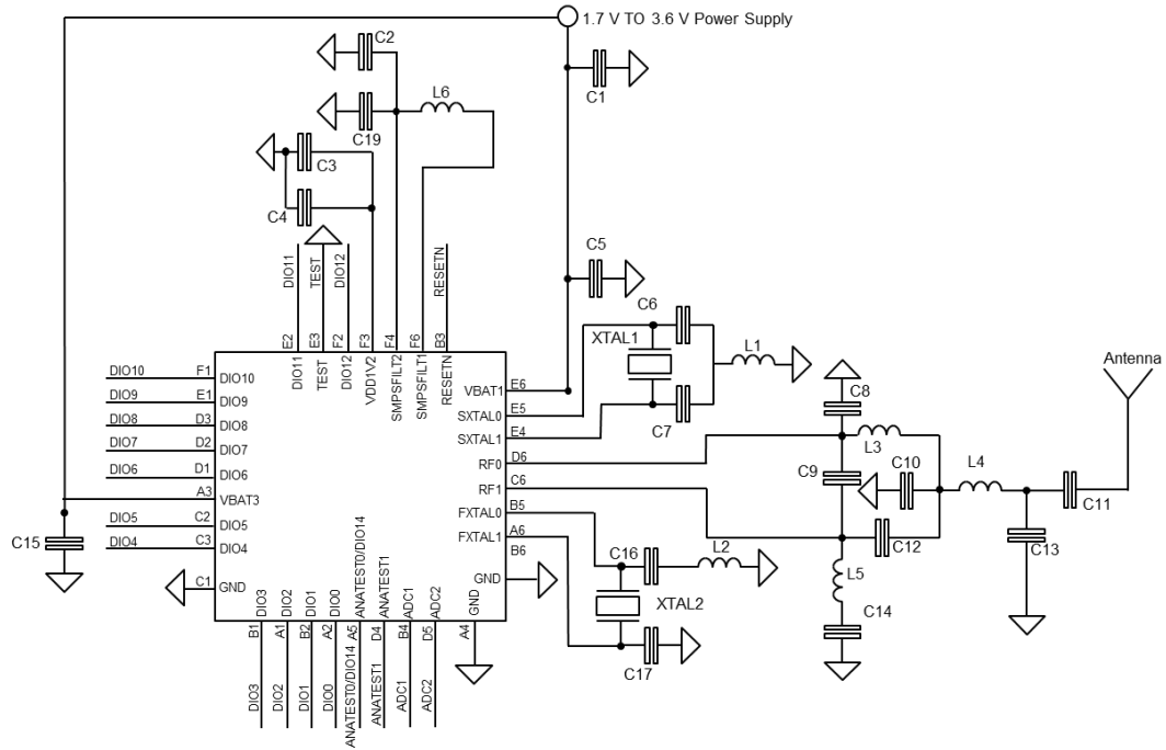
Figure 26. Application circuit: active DC-DC converter WLCSP34 package
