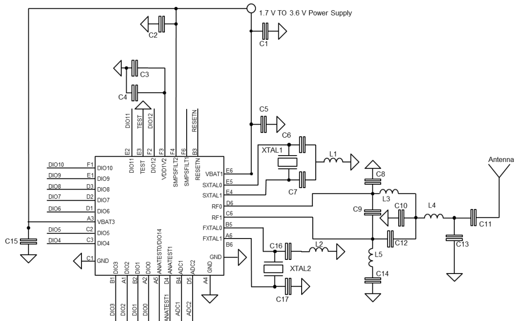
Figure 27. Application circuit: nonactive DC-DC converter WLCSP34 package
