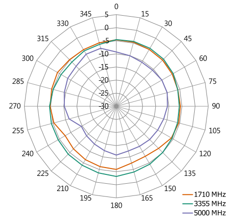
XY-Plane Gain
