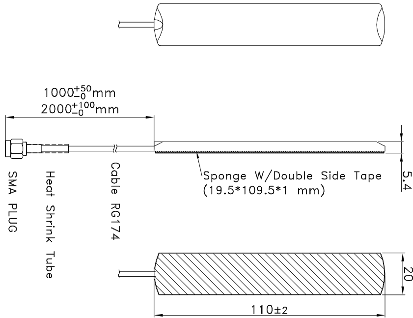
Figure 2. Antenna Dimensions
