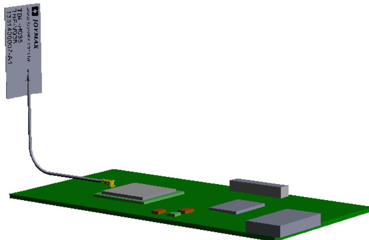
Figure 3. Antenna Installation
