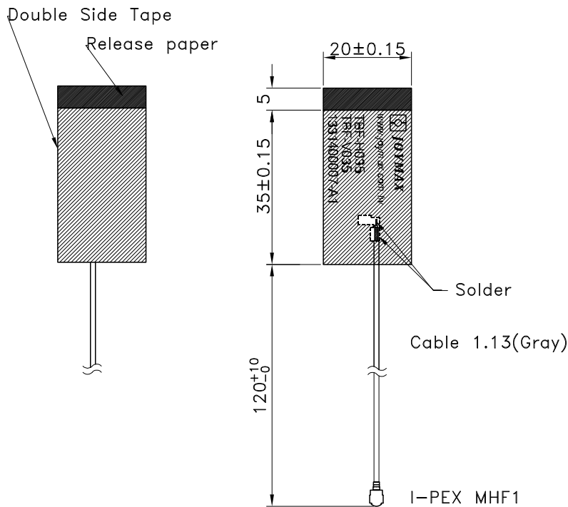
Figure 2. Antenna Dimensions
