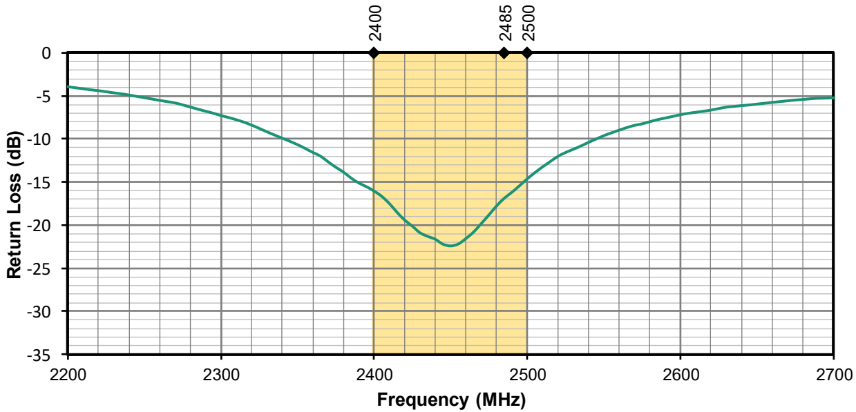
Figure 6. Antenna Return Loss, Straight, No ground plane
