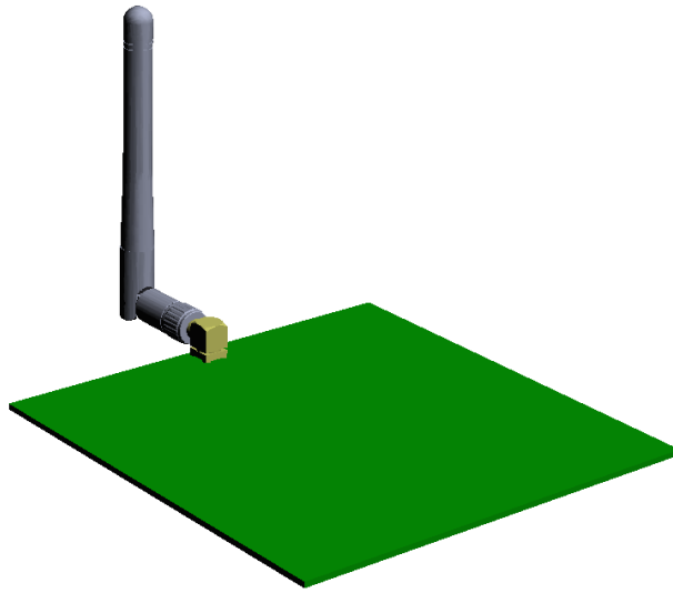
Figure 11. On edge of ground plane, Bent 90 Degrees
