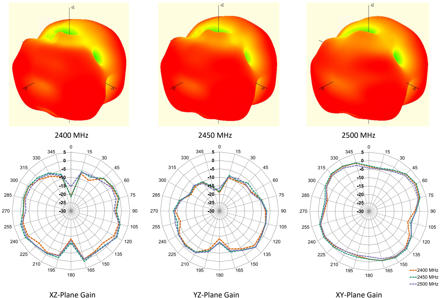
Figure 9. Antenna Radiation Patterns, with ground plane
