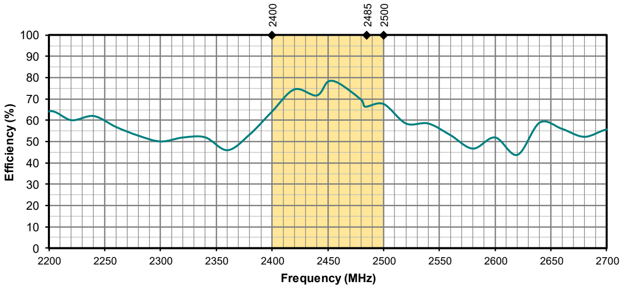
Figure 8. Antenna Efficiency, with ground plane
