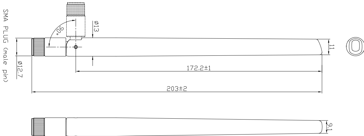
Figure 2. Antenna Dimensions
