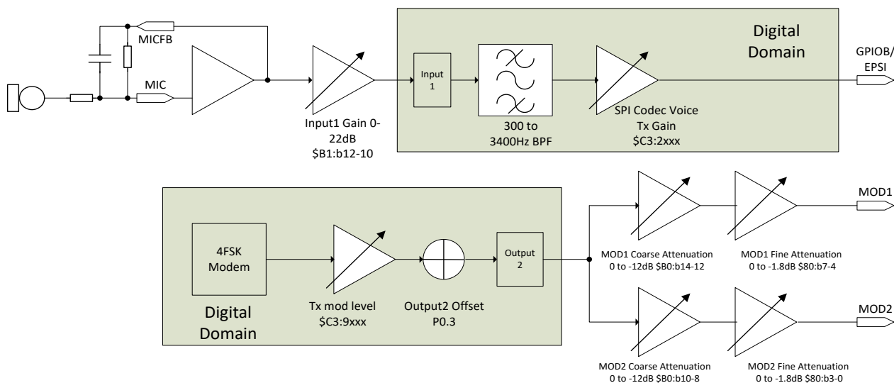
Figure 34 Tx Levels
