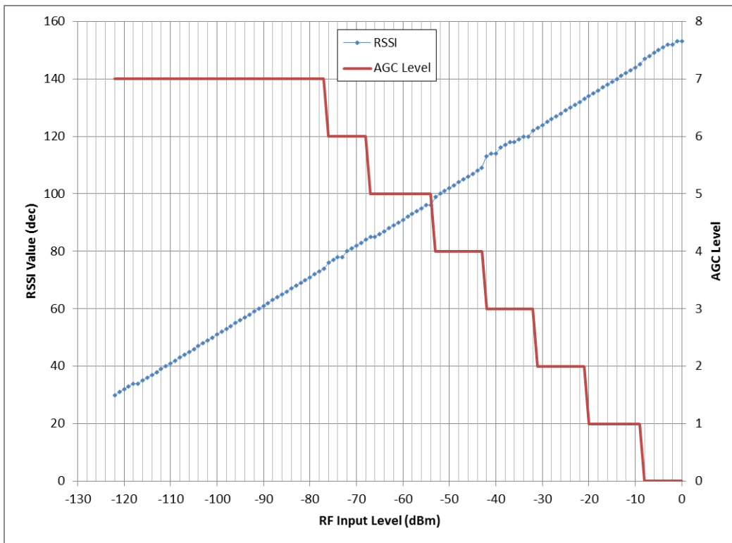
Figure 8 RSSI/AGC in I/Q Mode
