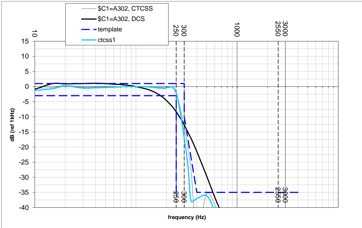
Figure 30 CTCS and DCS filters
