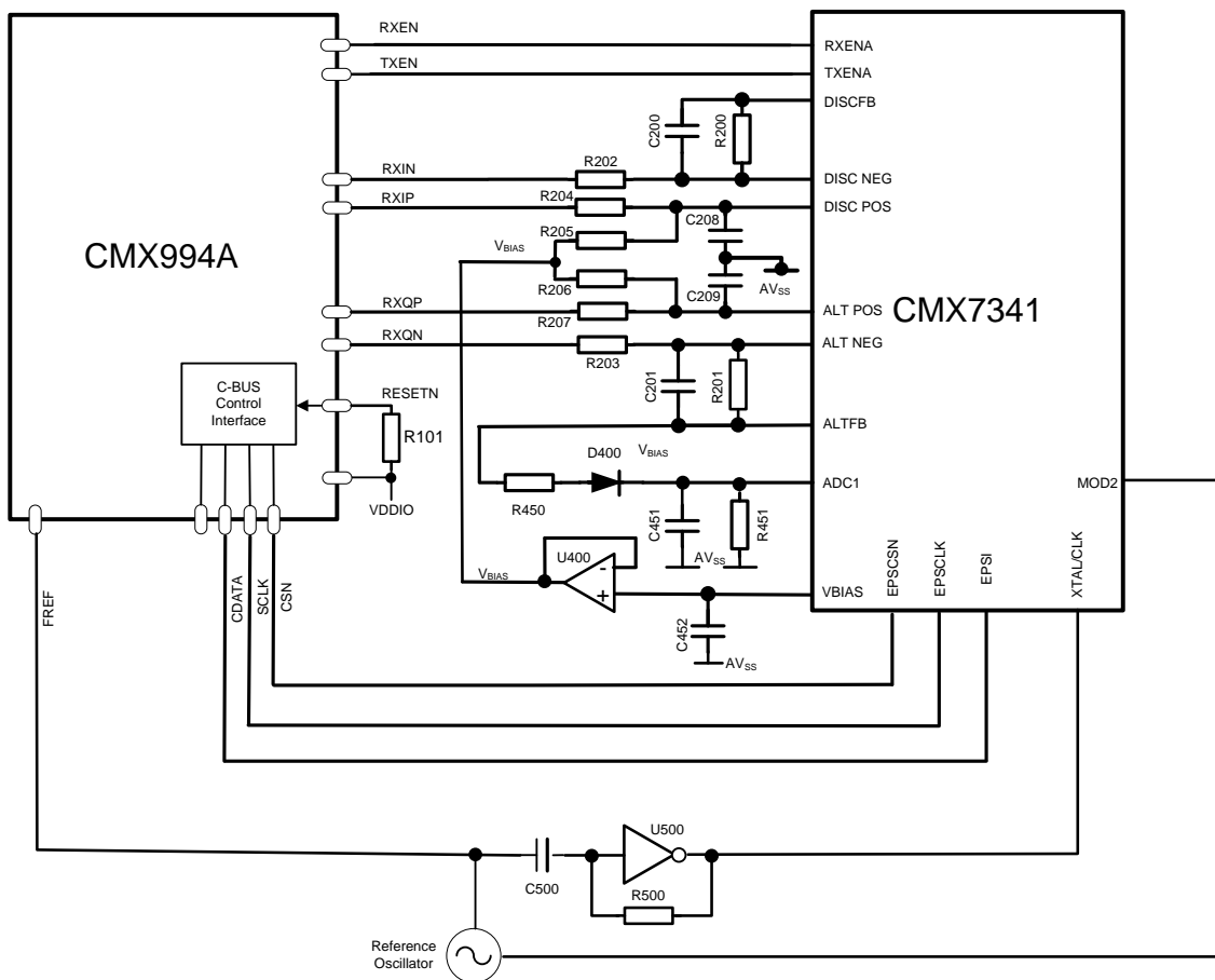
Figure 6 CMX7341/CMX994A Interface
