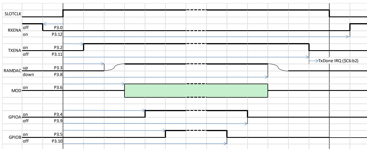
Figure 23 Tx Sequencer Delay Timers
