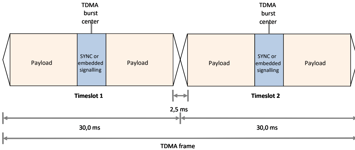
Figure 11 MS Sourced TDMA Frames
