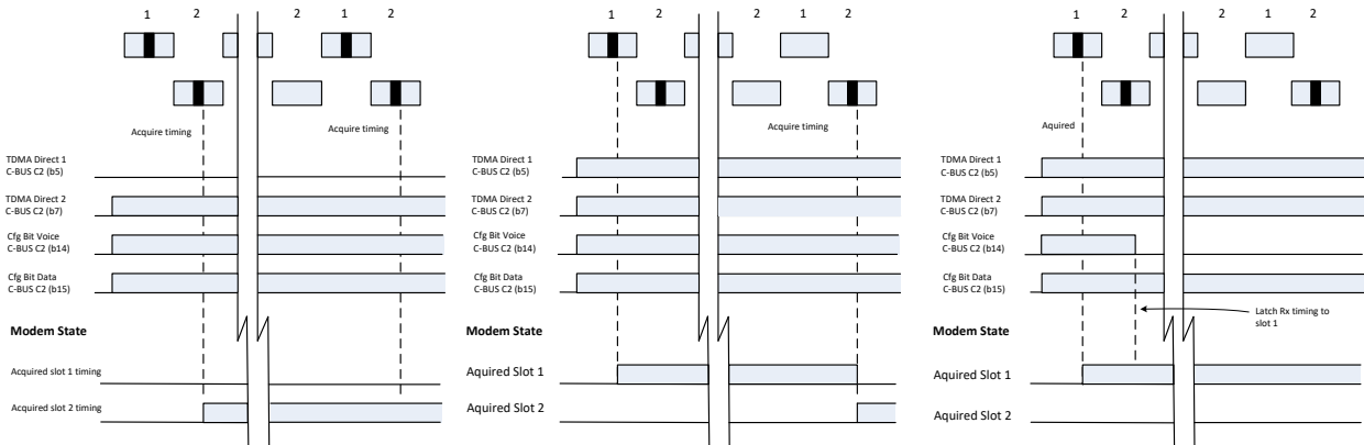
Figure 20 Timing Scenarios
