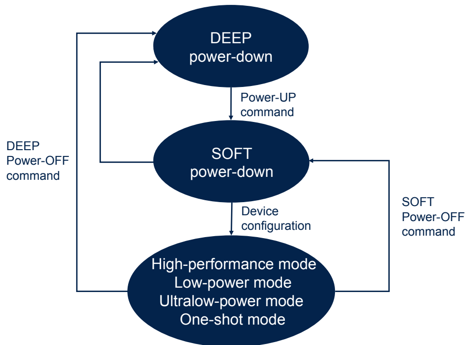
Figure 6. Power-up sequence
