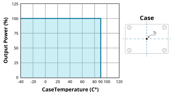
CASE TEMPERATURE (Tc) DERATING CURVE
