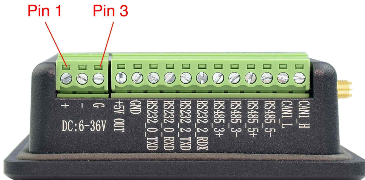
Power Input
