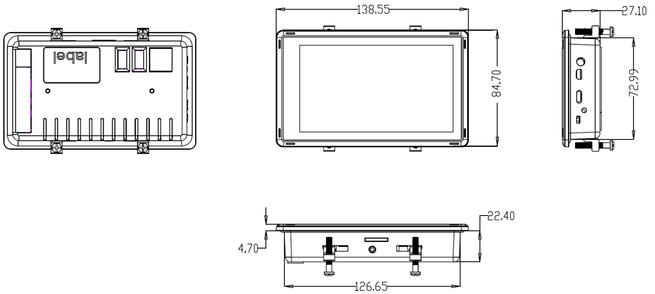
Technical Drawing
