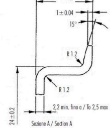
Profilato a cappello TH 35-15 Top hat rail TH 35-15
