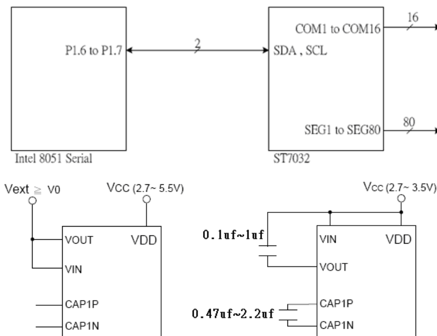
Intel 8051 interface( I 2 C )
