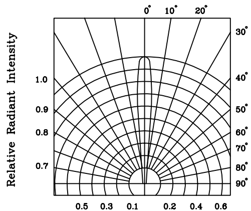
FIG.6 RADIANT DIAGRAM
