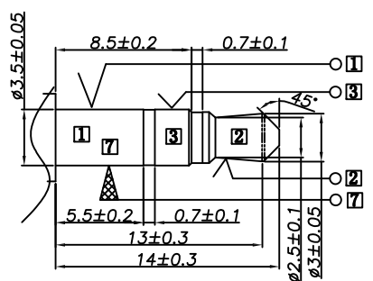
MATE PLUG
