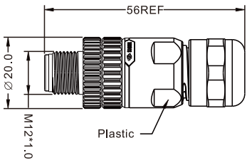
Scale Diagram
