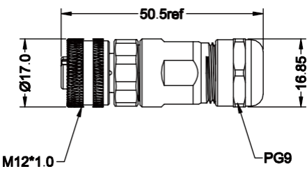
Scale Diagram
