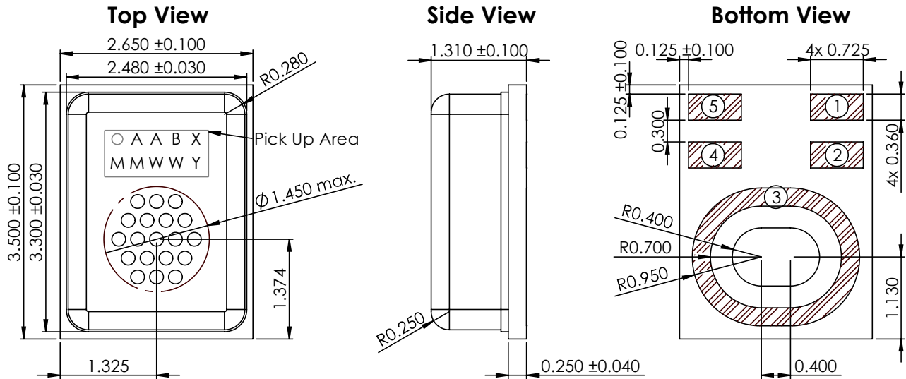
Figure 8.1: Mechanical drawings (mm)
