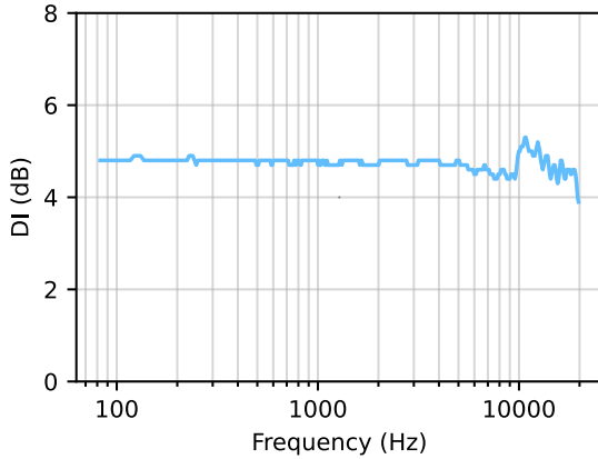
Figure 7.3: Directivity index vs frequency
