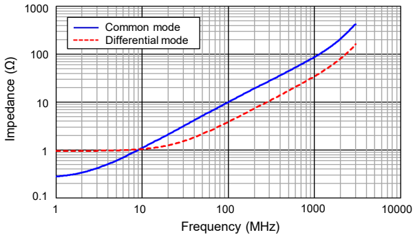
[ Impedance characteristics ]
