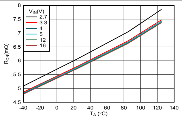
Figure 7-3. ON-Resistance vs Temperature ( I_{\text{OUT}} = 3\text{ A} )
