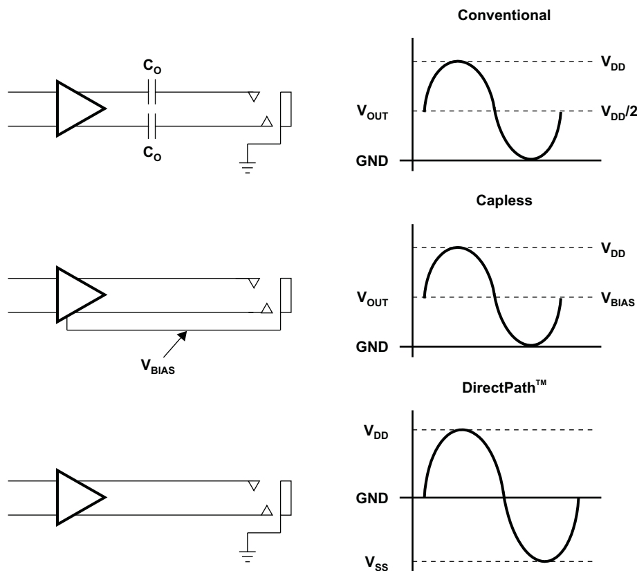
Figure 64. Amplifier Applications
