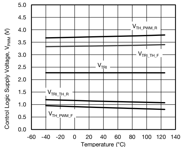
Fig. 14 - PWM Threshold vs. Temperature (SiC638)
