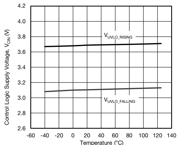
Fig. 12 - UVLO Threshold vs. Temperature
