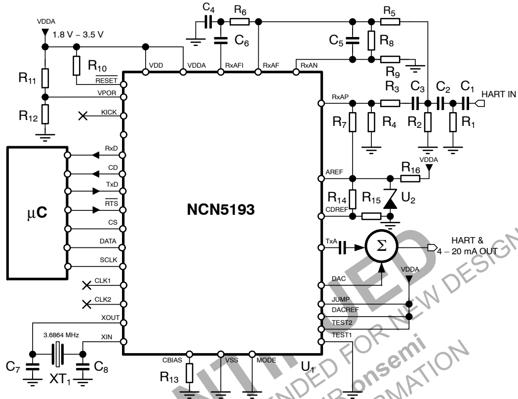
Figure 2. Application Diagram NCN5193
