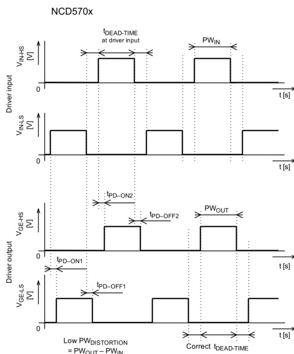
Figure 23(b). NCD5700 Timing Waveforms
