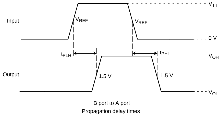
Figure 7. Voltage Waveforms
