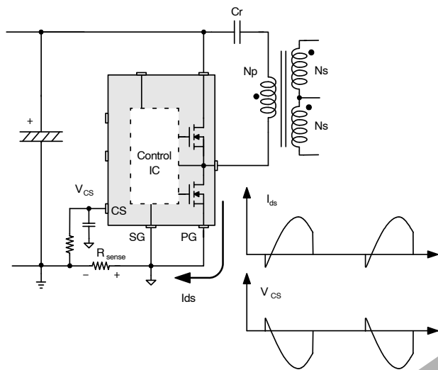
Figure 24. Half-Wave Sensing
