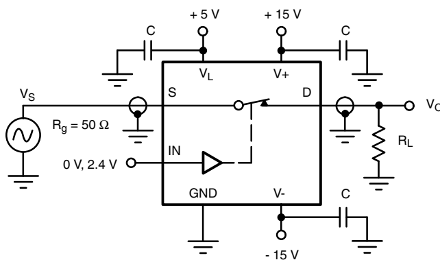
Fig. 8 - Insertion Loss
